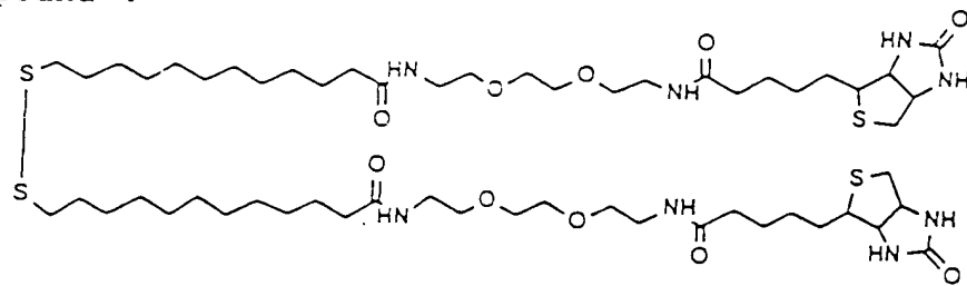
biotin compound 4
